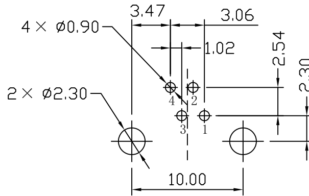
PC Board Layout (Top View)
