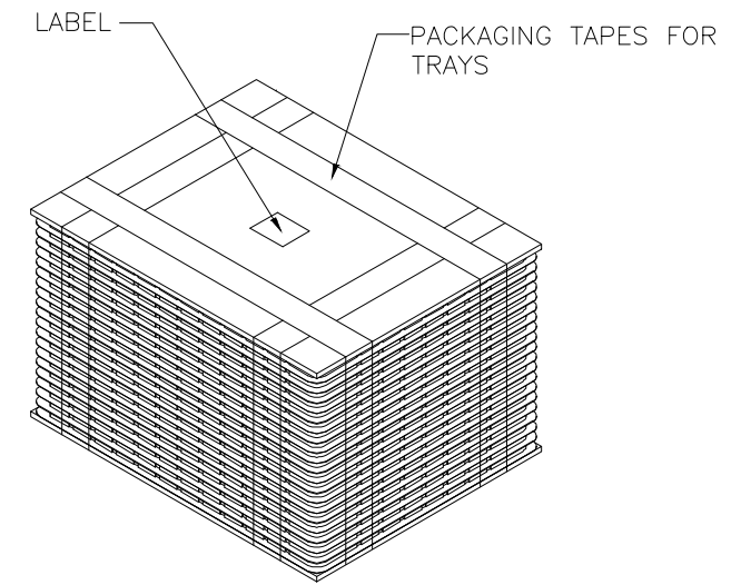
3. LABEL & PACKAGING TAPES FOR TRAYS:
