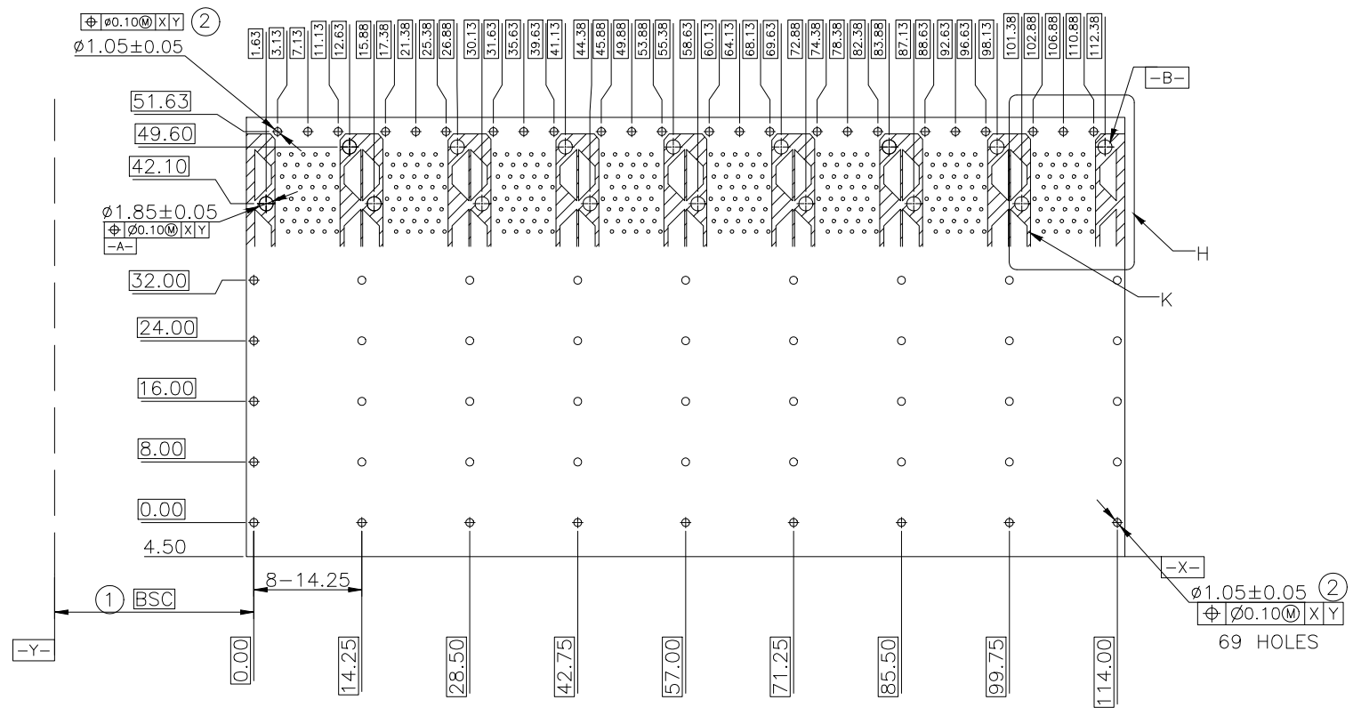
RECOMMENDED PCB CONFIGURATION
