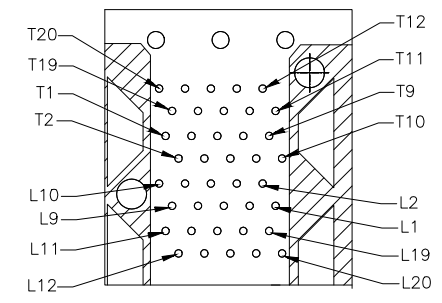
CONNECTOR PIN-OUT COMPONENT SIDE OF BOARD
