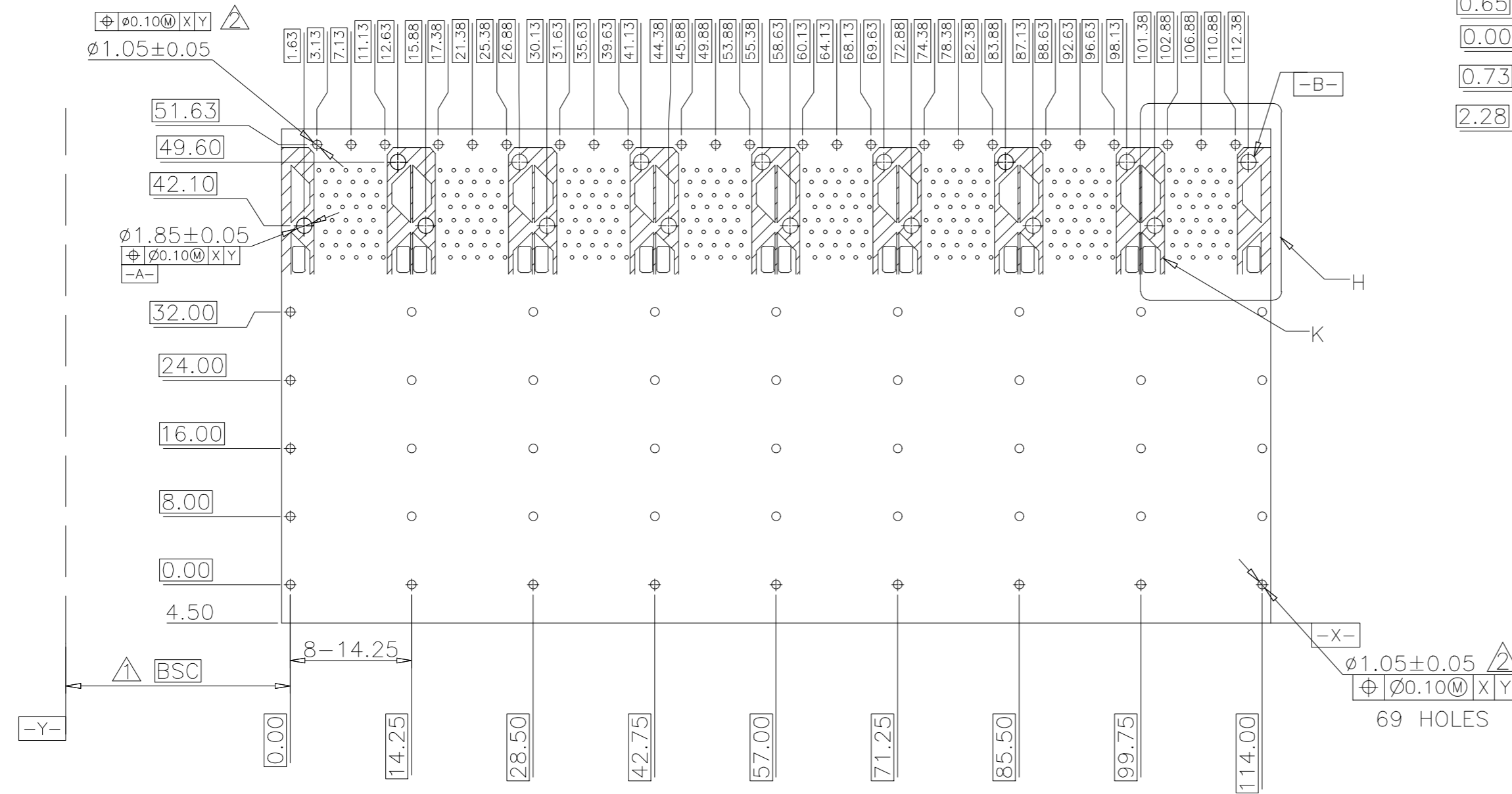
RECOMMENDED PCB CONFIGURATION
