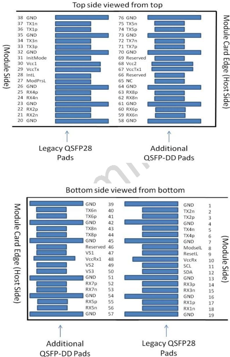
Figure 1. Host PCB QSFP-DD pad assignment top view
